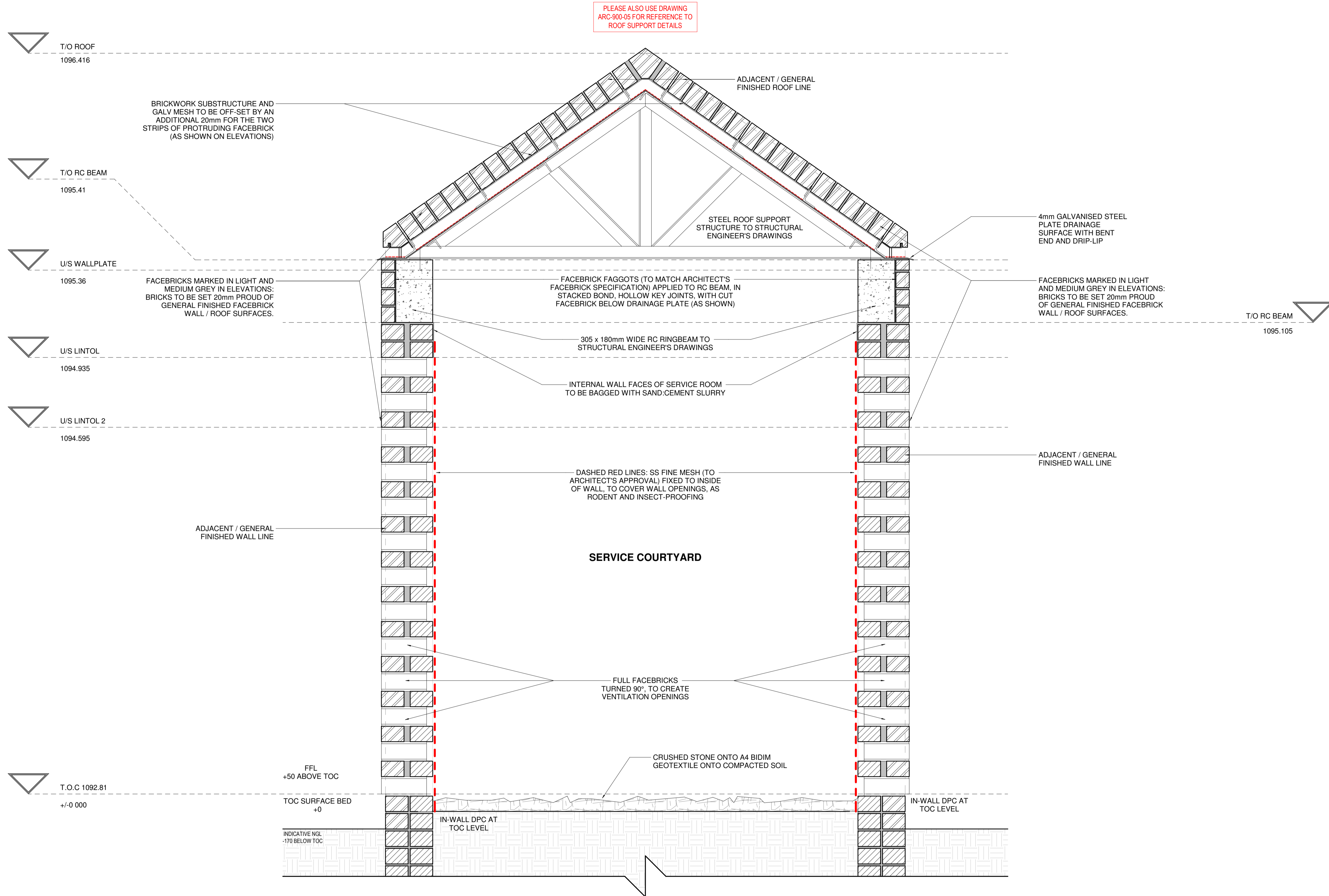
200.04_BRISE-SOLEIL DETAILS_SECTION
